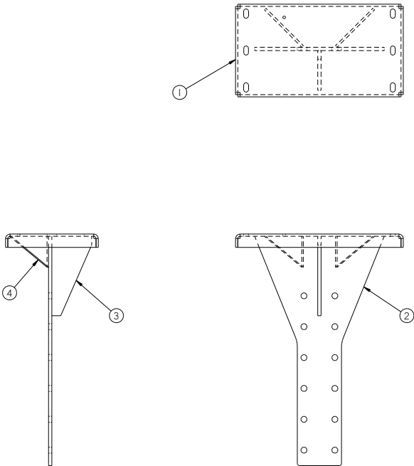
Figure 9.1323 51253 Front Leg Support Mounting Plate Assembly
