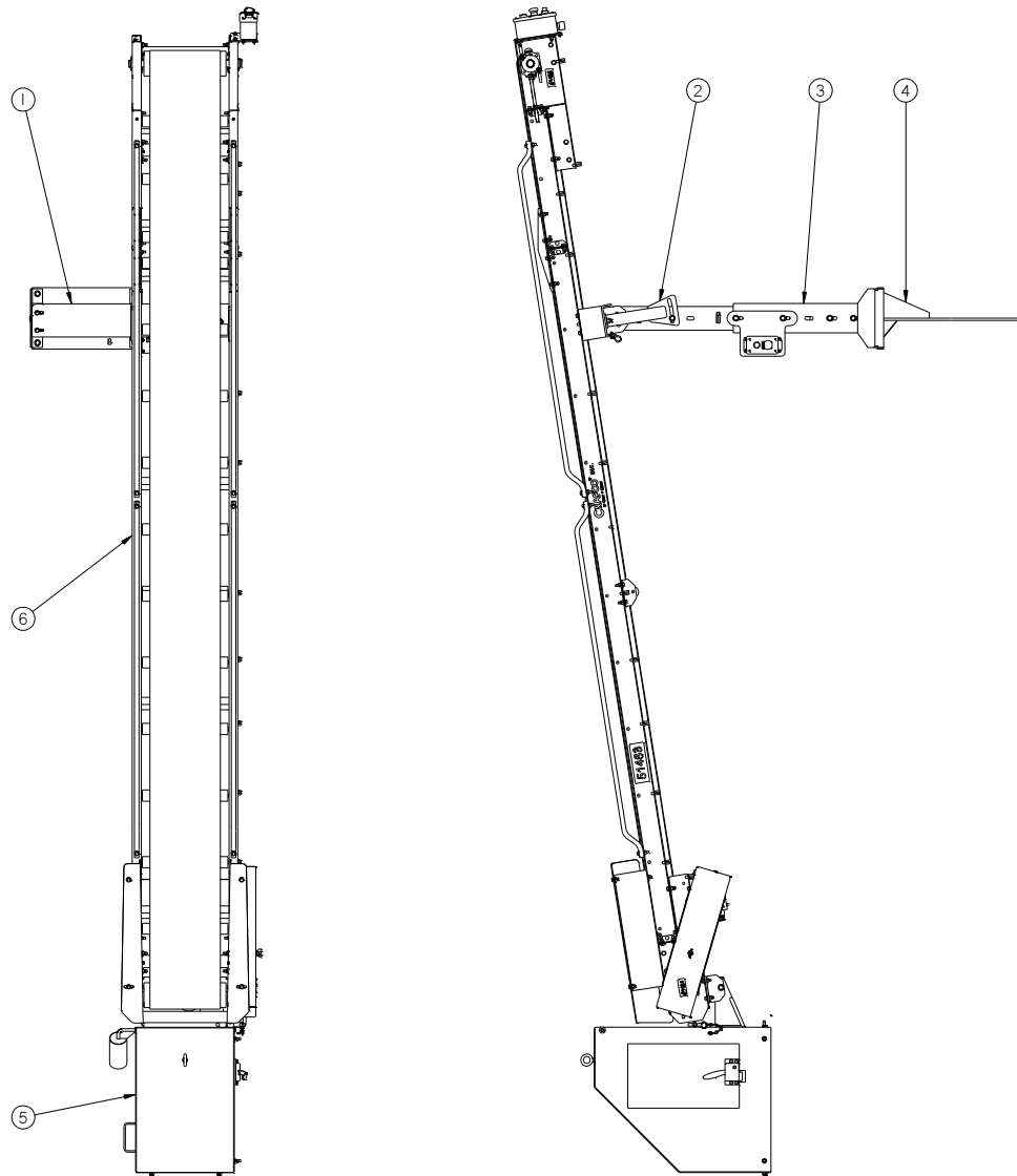
Figure 9.10 Super Shot 250 Diesel and Diesel Compressor Melter Autoloader Kit
