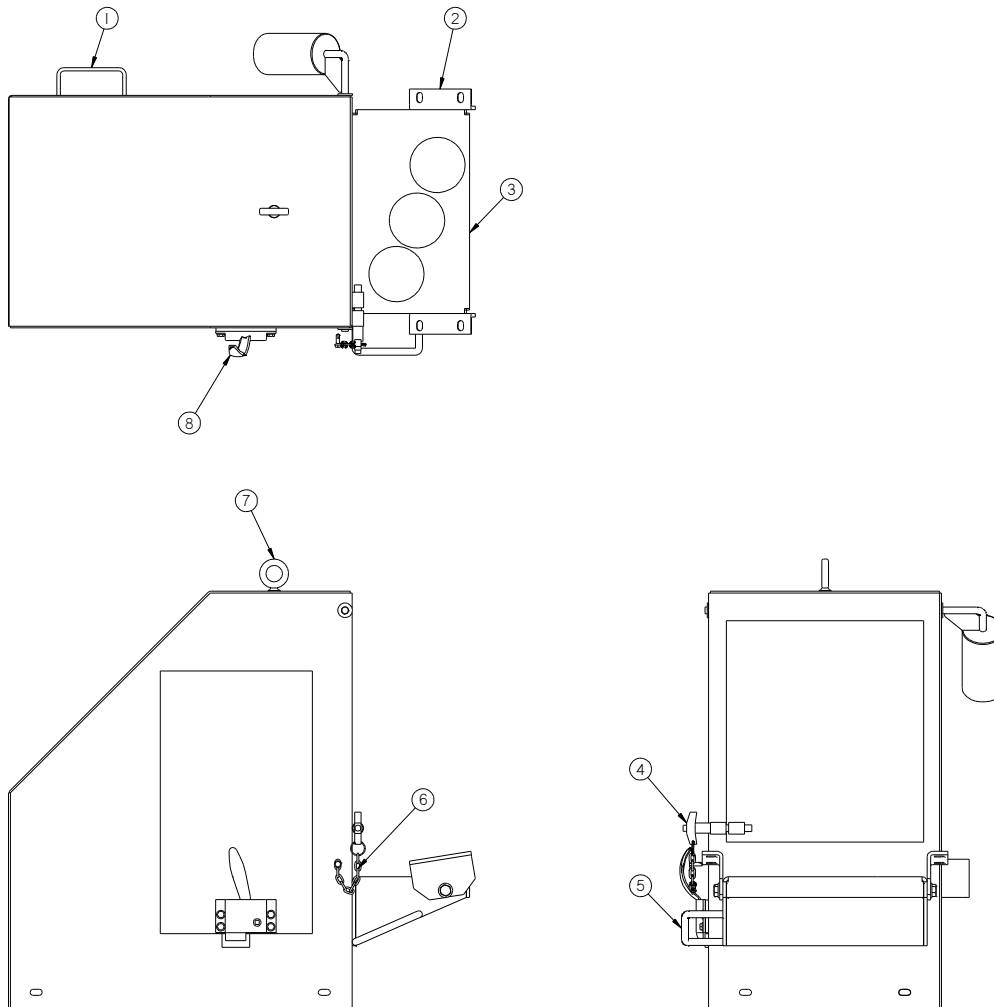
Figure 9.15 51370 Splash-Box-Welded-Assembly
