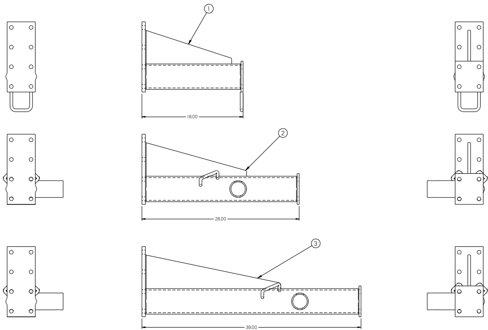
Figure 9.3350 Hitch Extension Options
