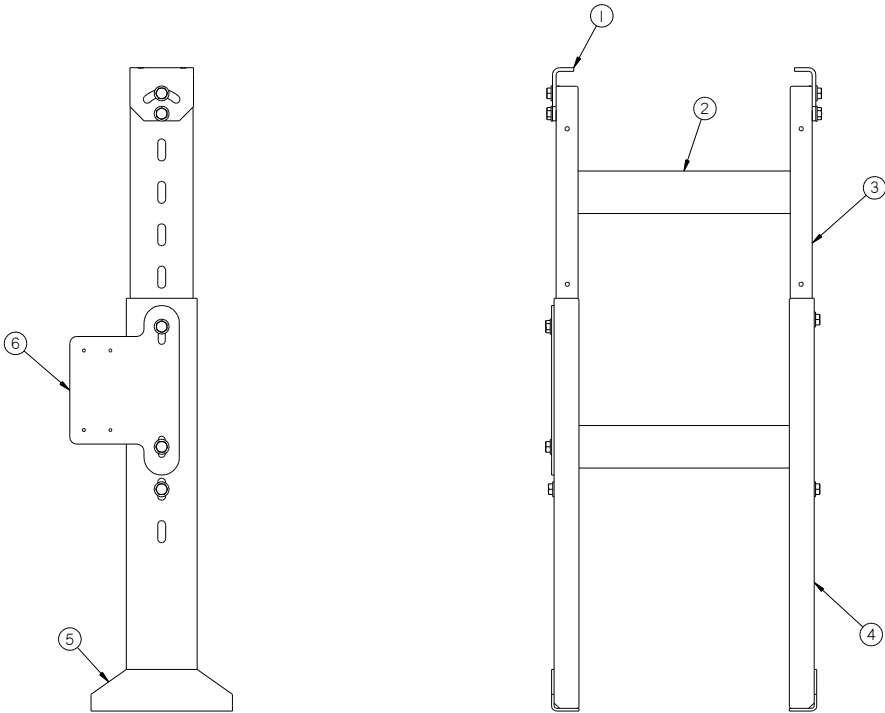
Figure 9.32 51113 Heavy-Duty Structure Support
