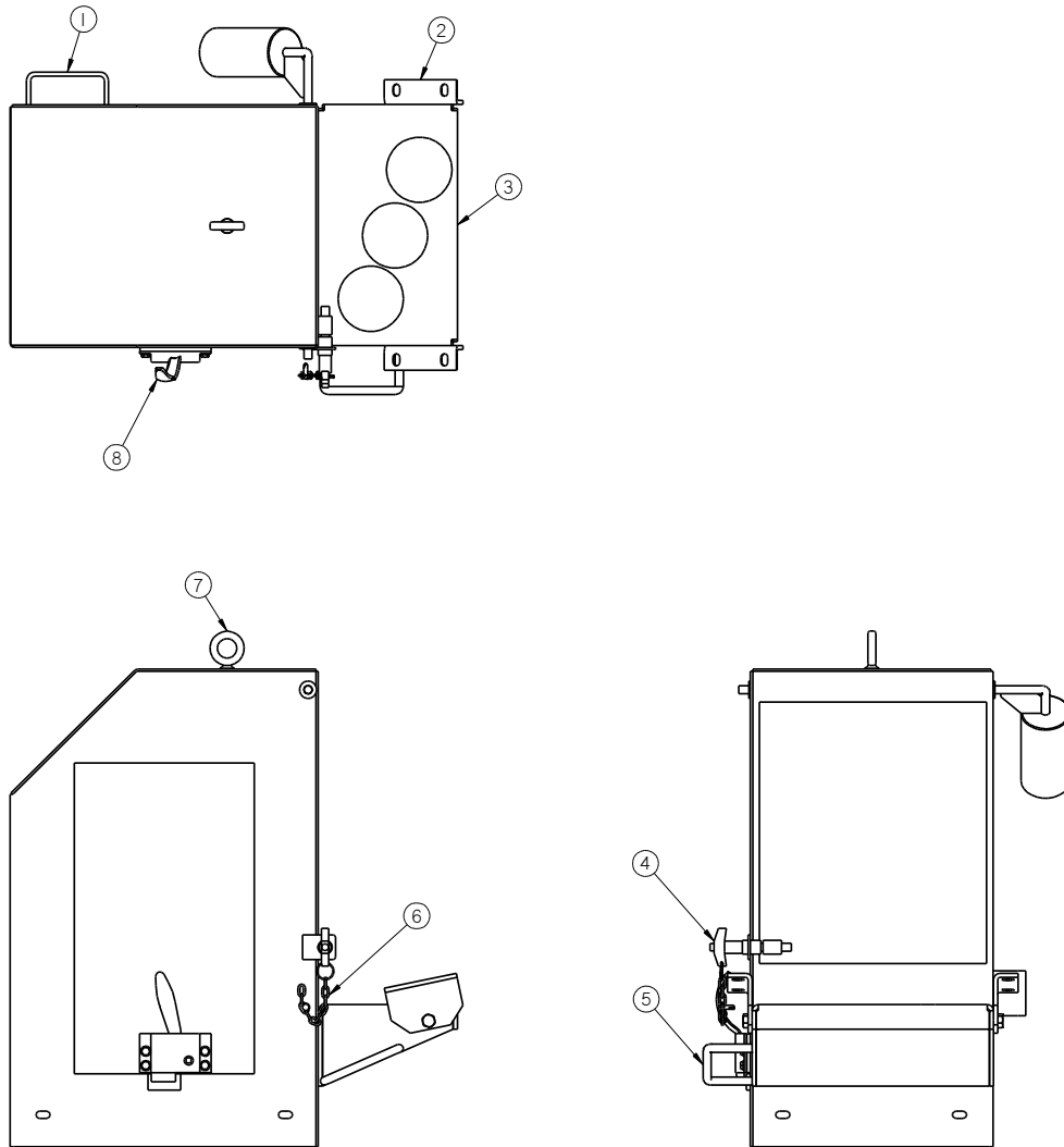
Figure 9.5 51320 Splash Box Welded Assembly
