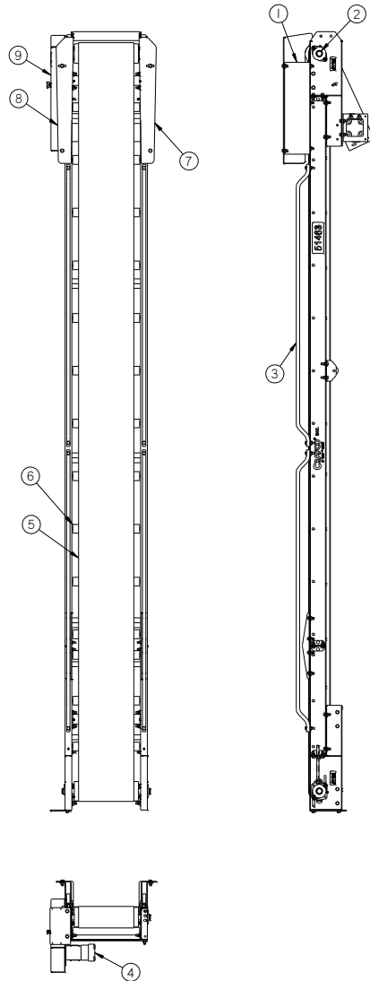
Figure 9.16 51429 12' Conveyor Assembly
