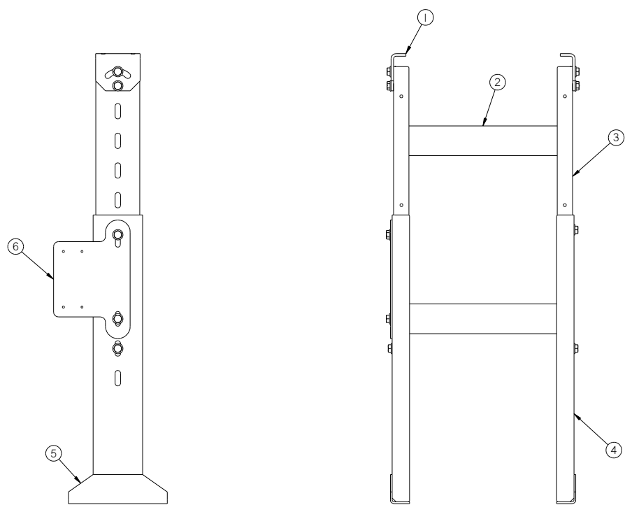
Figure 9.2342 51113 Heavy Duty Structure Support
