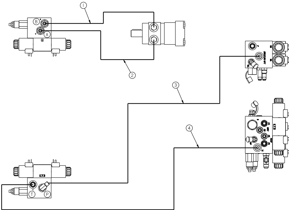
9-38-26609-Hydraulic Schematic EZ-Series II-1000-Autoloader
