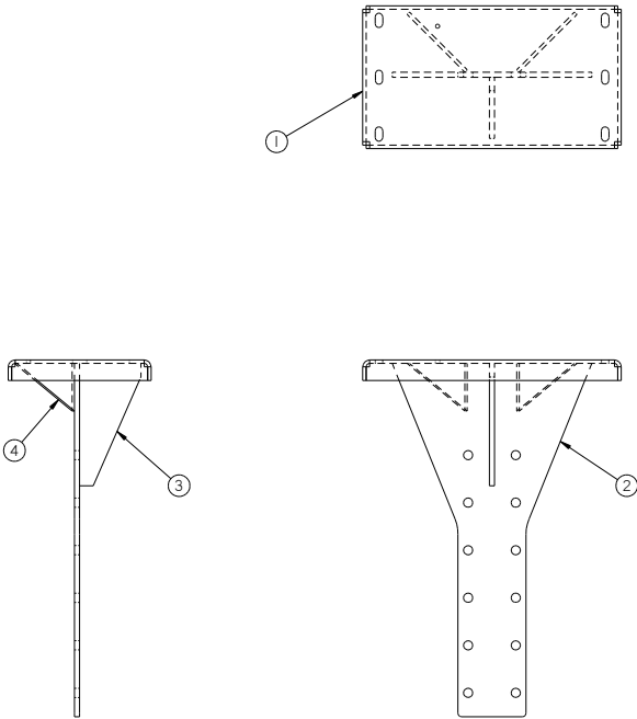
Figure 9.2443 51253 Front Leg Support Mounting Plate Assembly
