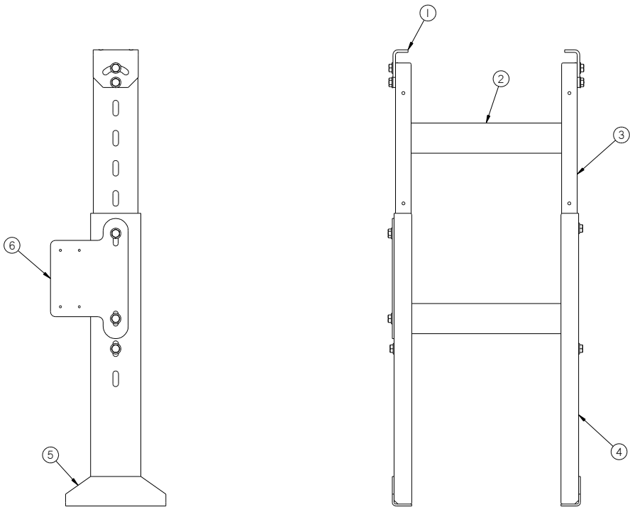
Figure 9.3 51113 Heavy Duty Structure Support
