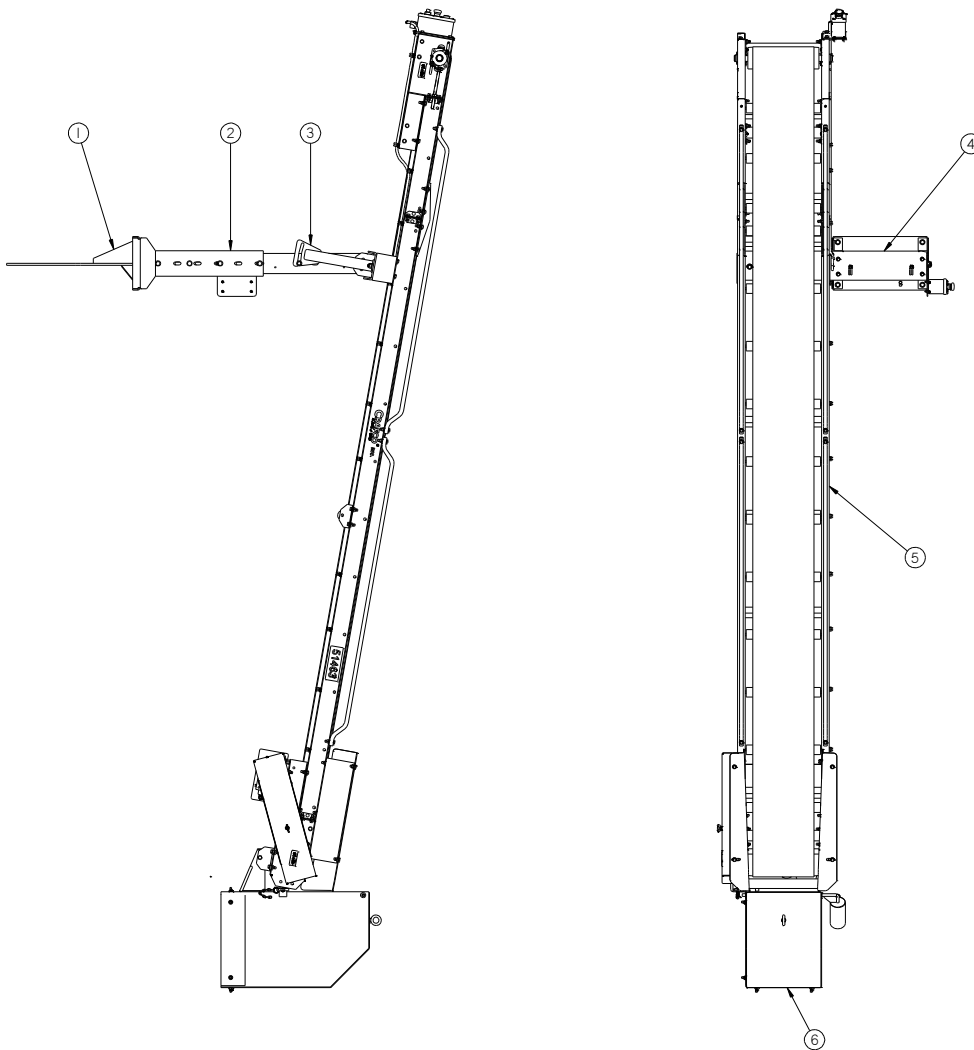
Figure 9.29 EZ Series II 1000 Diesel and Diesel Compressor Melter Autoloader Kit
