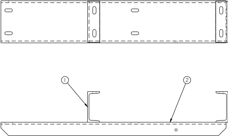
Figure 9.2 51302 Top Support-Cross Over Assembly
