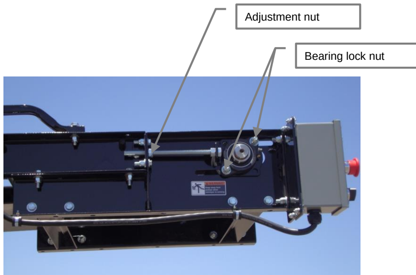
Figure 6.1 Belt Tracking Adjustment
