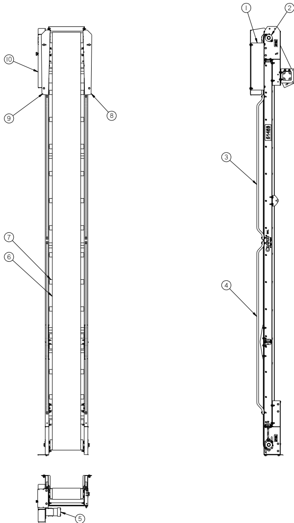
Figure 9.1525 51430 13' Conveyor Assembly
