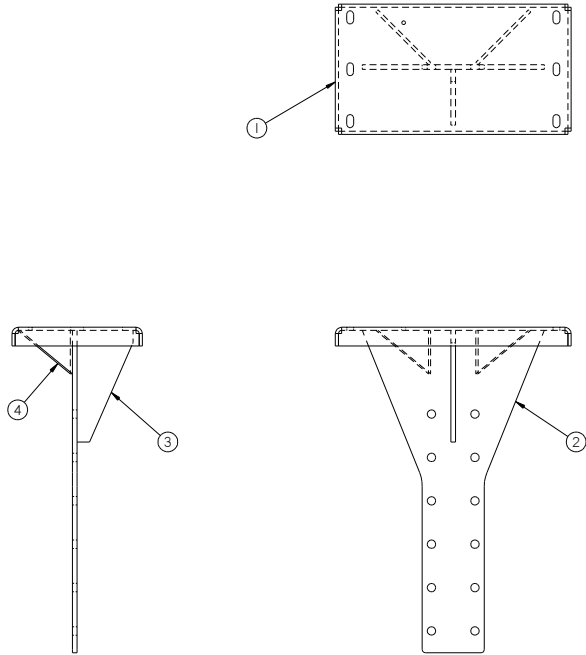
Figure 9.14 51253 Front Leg Support Mounting Plate Assembly
