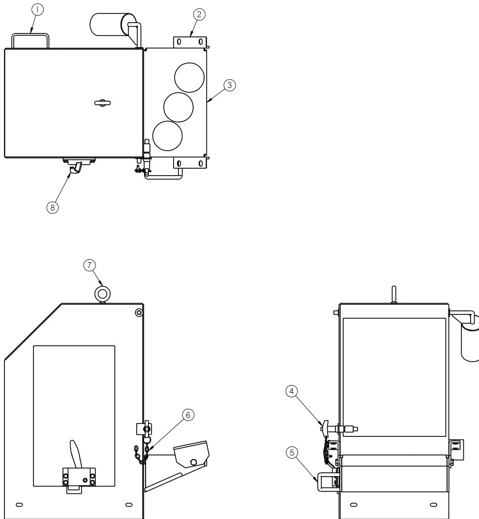
Figure 9.1424 51320 Splash Box Welded Assembly
