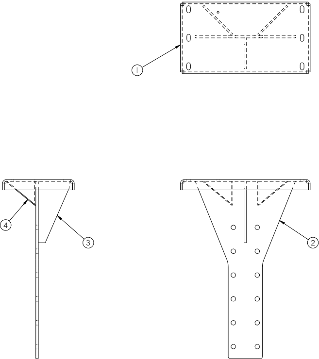
Figure 9.4 51253 Front Leg Support Mounting Plate Assembly
