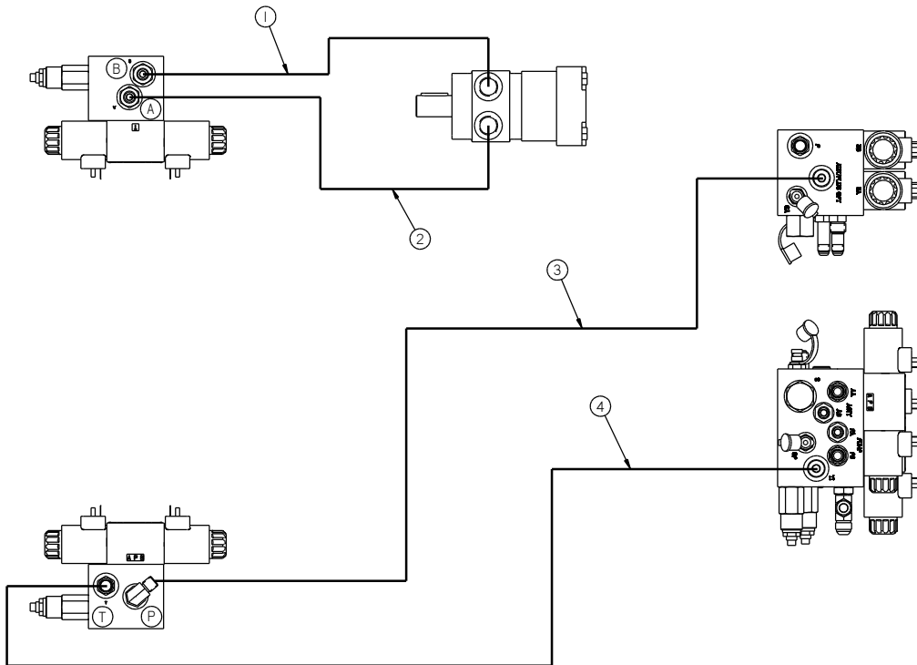
Figure 9.3049 26605 Hydraulic Schematic EZ Series II 1500 Autoloade
