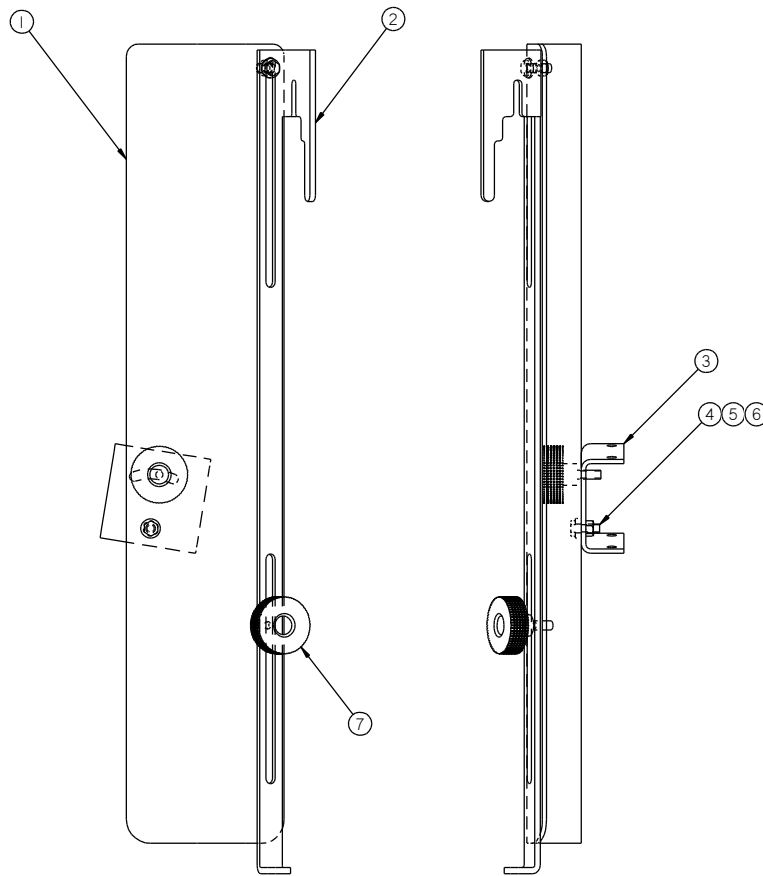
Figure 9.2746 46614 Boom Lock Assembly Conveyor
