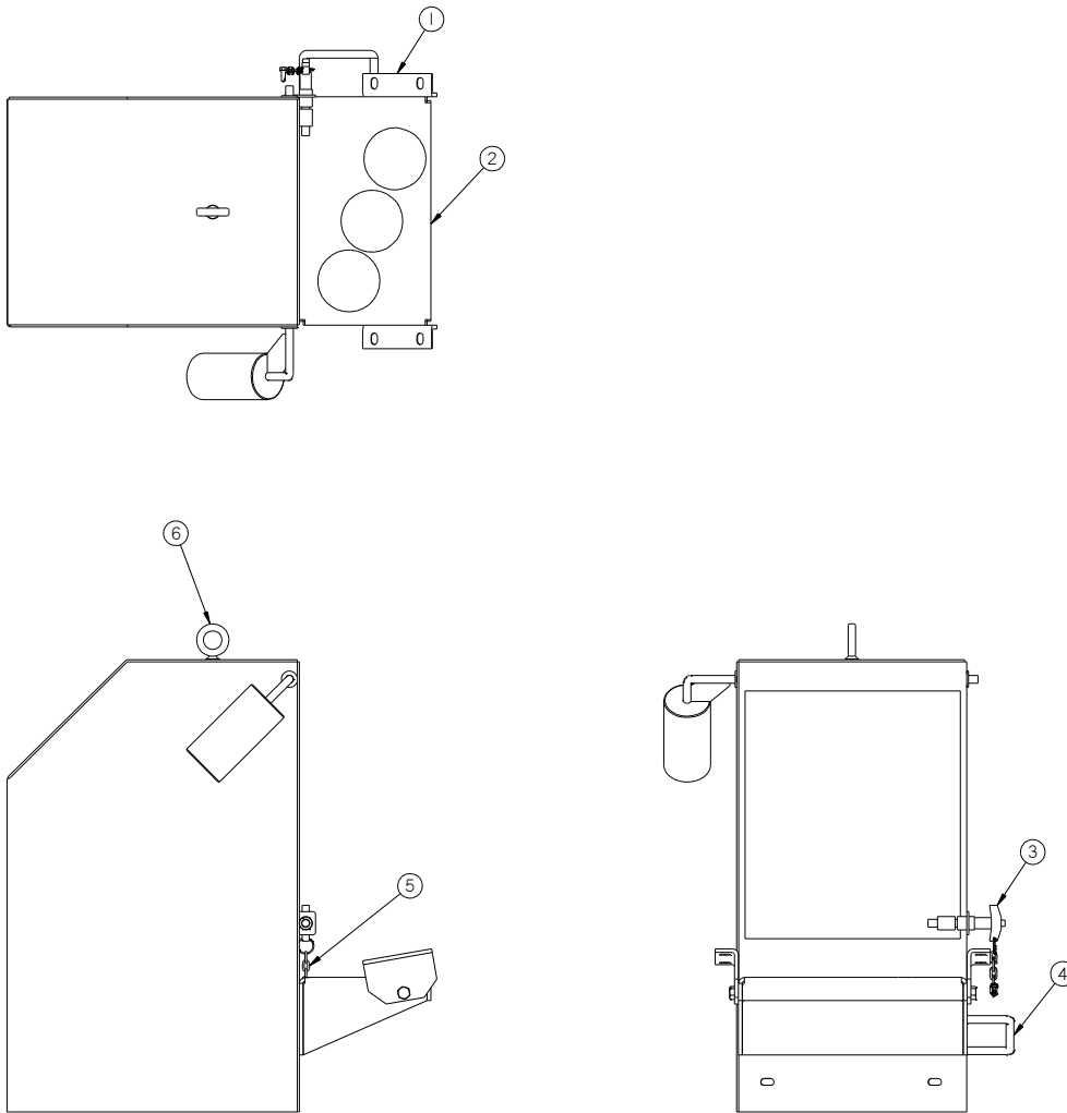
Figure 9.2544 51375 Splash Box Welded Assembly LH
