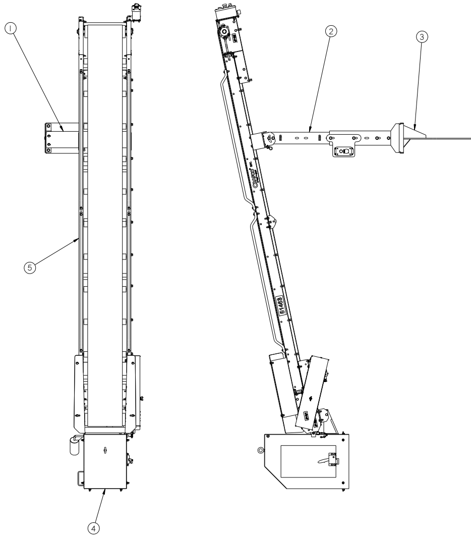
Figure 9.1 51177 Super Shot 125 Diesel and Diesel Compressor Melter Autoloader Kit
