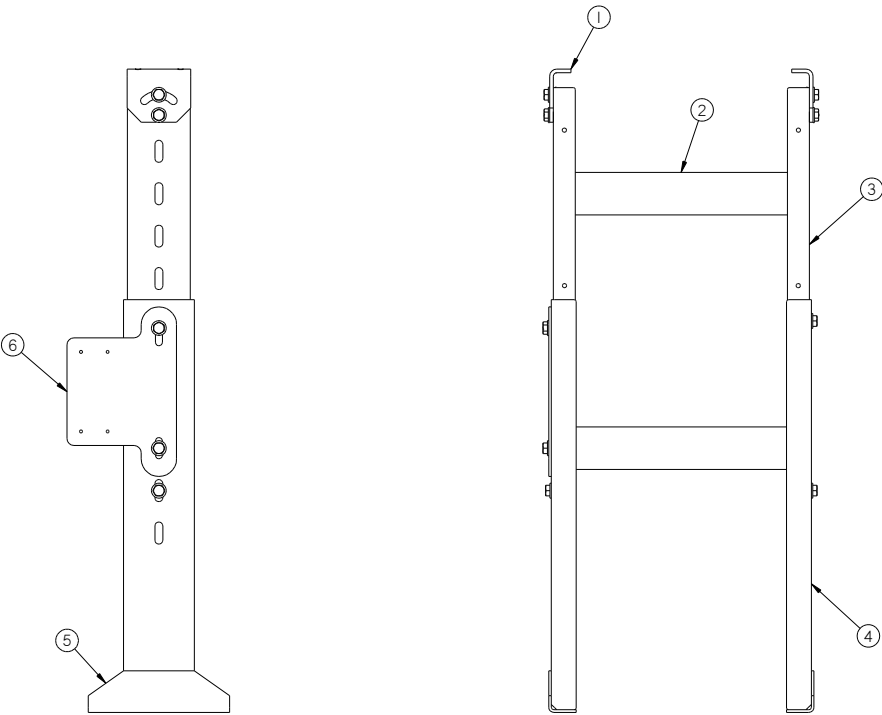
Figure 9.13 51113 Heavy Duty Structure Support
