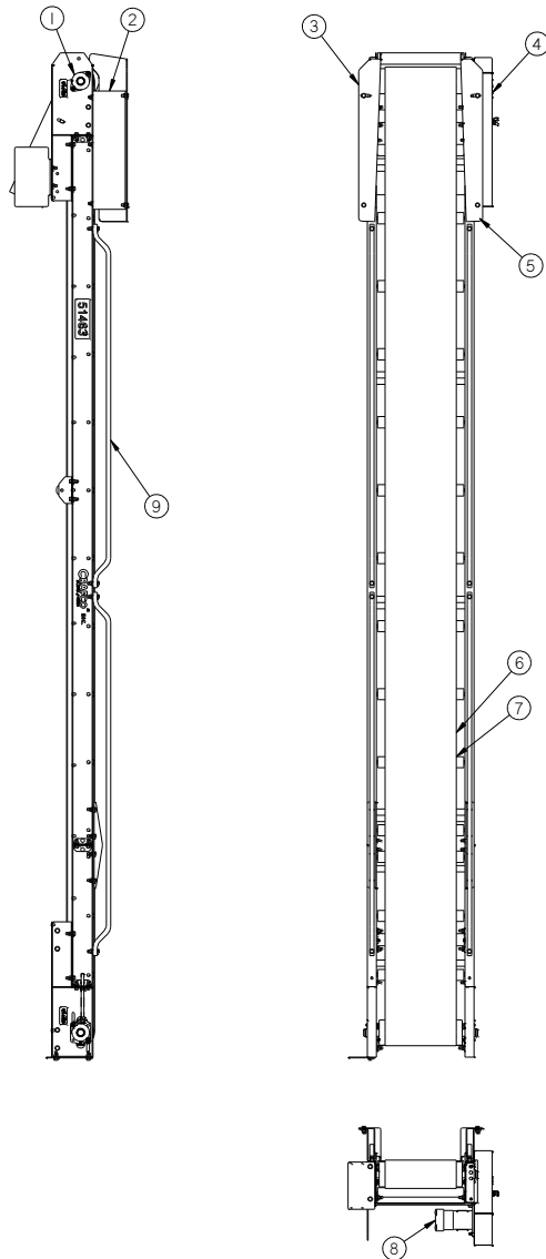
Figure 9.2645 5144068 123' Conveyor Assembly
