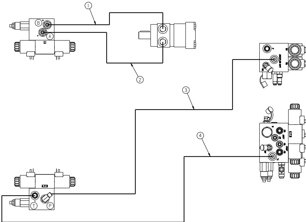
9-289.18 26608 Hydraulic Schematic EZ Series II 500 (All Models) Autoloader
