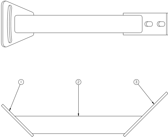
Figure 9.30 51255 Underbody Angled Support Brace
