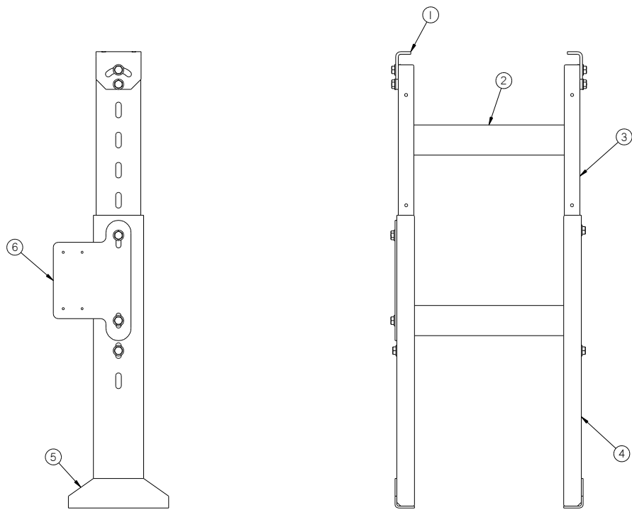
Figure 9.1222 51113 Heavy Duty Structure Support
