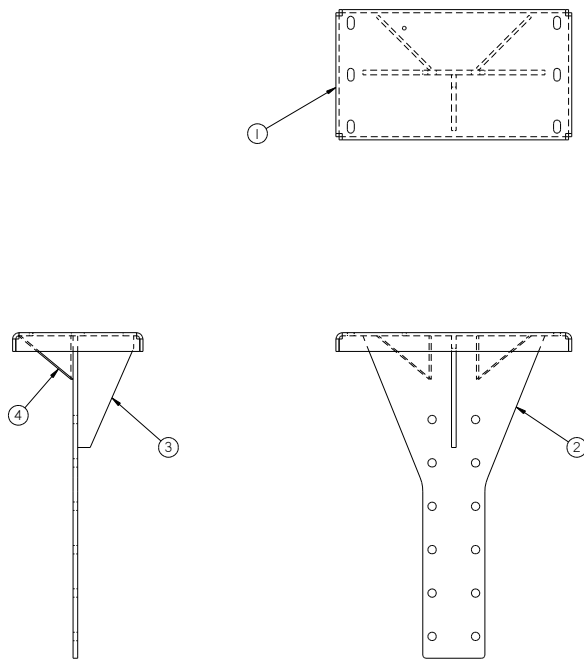
Figure 9.33 51253 Front Leg Support Mounting Plate Assembly
