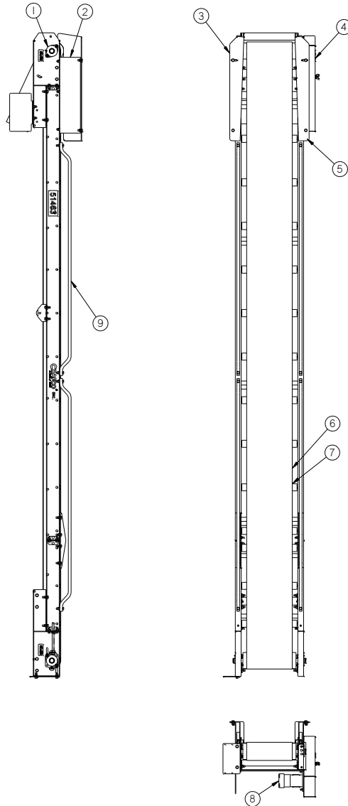
Figure 9.35 51440 12' Conveyor Assembly
